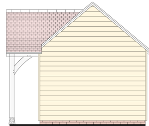
Right Hand Elevation
